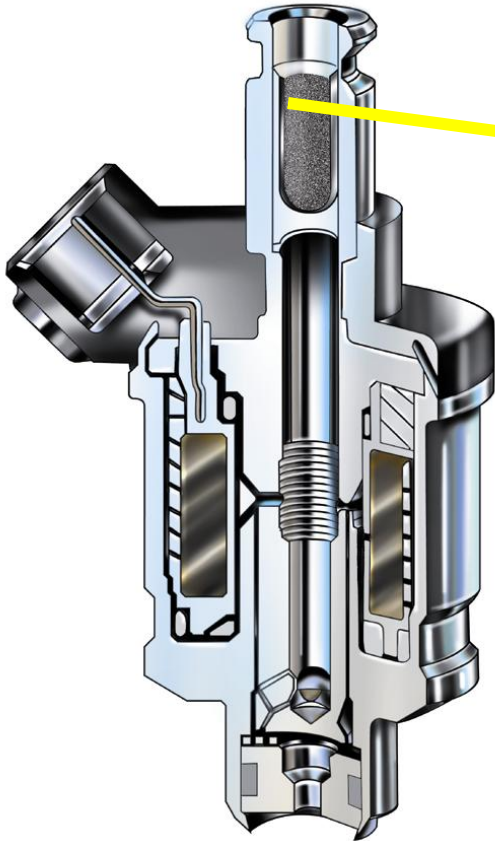
Honda-designed Fuel Injectors
