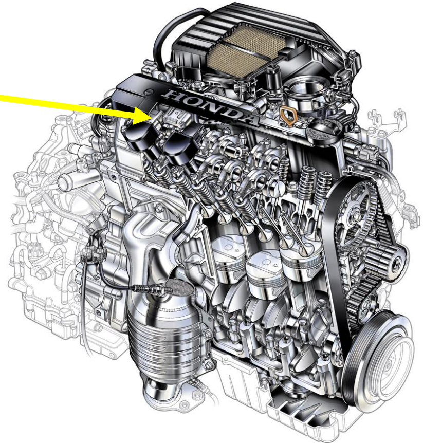
110-hp, 1.8-liter, 16- valve, SOHC i-VTEC 4-cylinder engine
